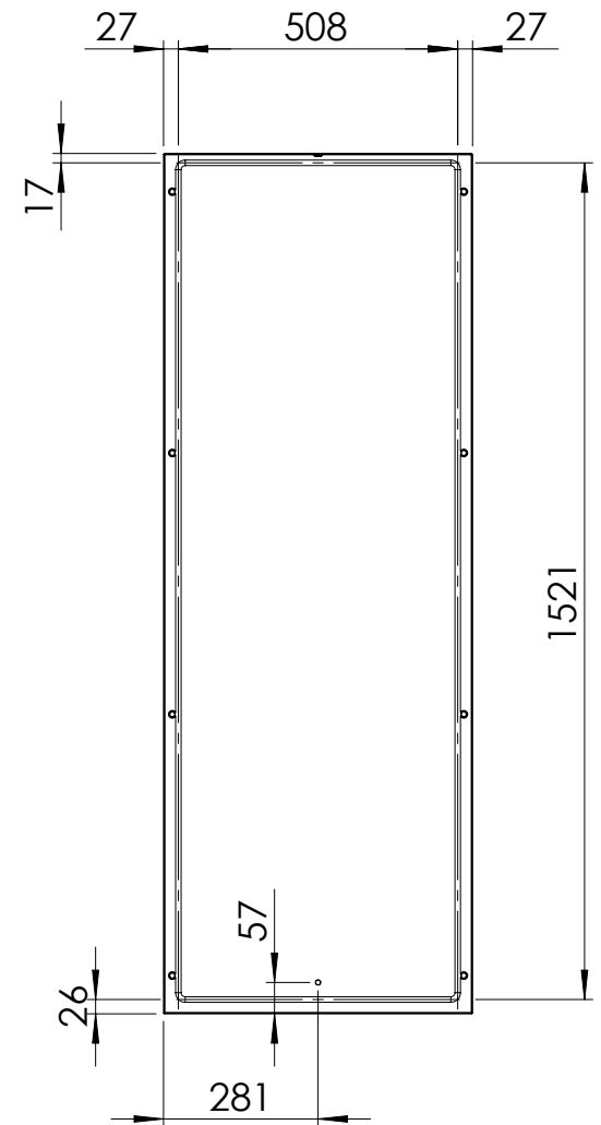
Rear view
