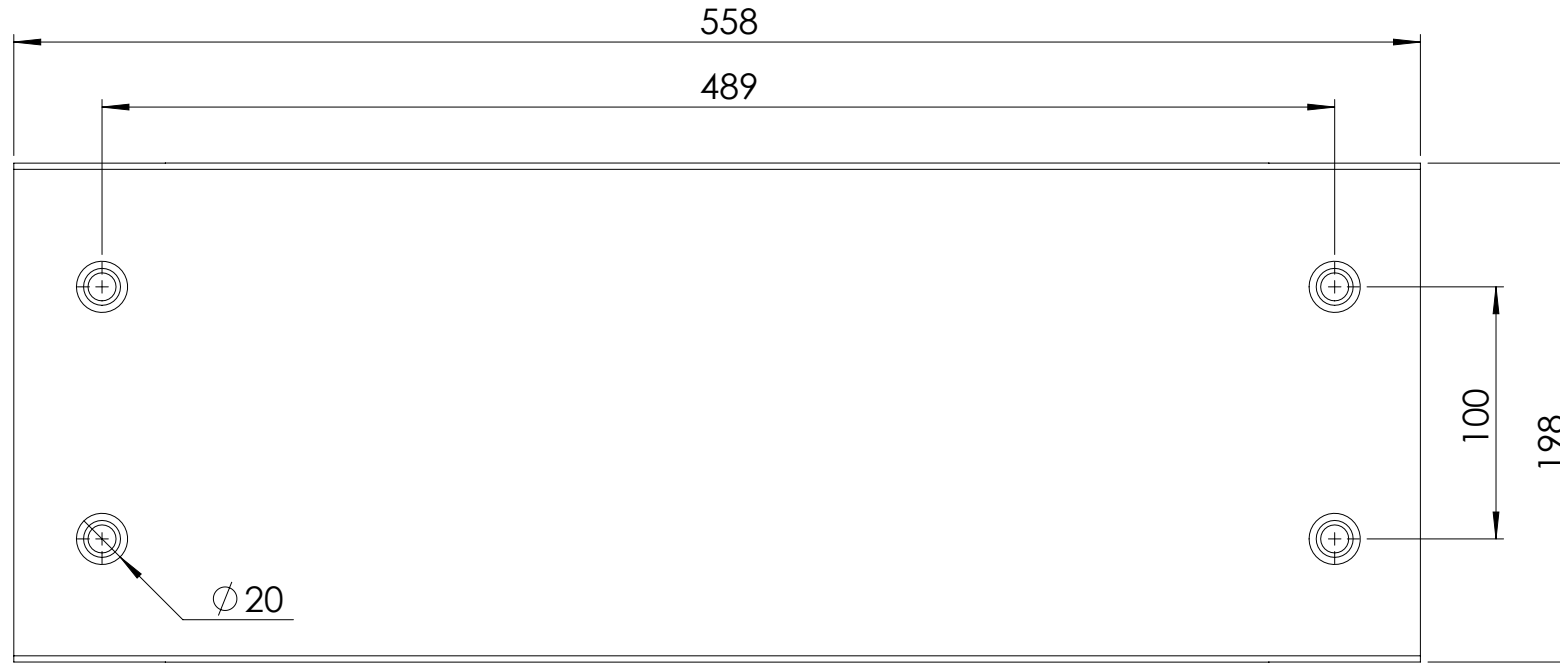
Top view
