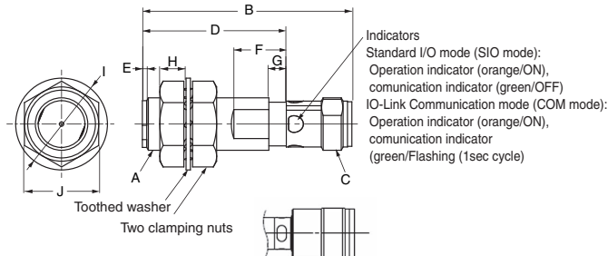
Model E2E(Q)-X□8-M1; Shape of connection.
