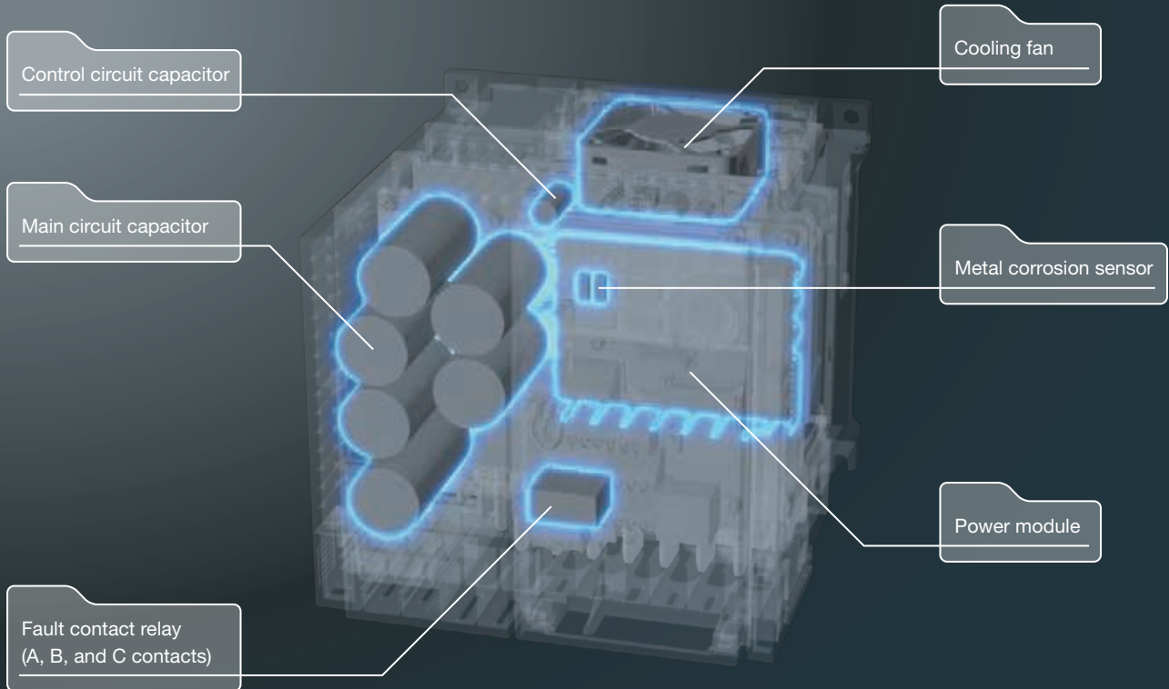
Example: FR-E840-3.7K
