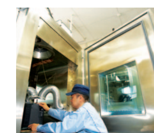
HALT Highly accelerated life test (HALT): Test to confirm the thermal and vibration limits.
