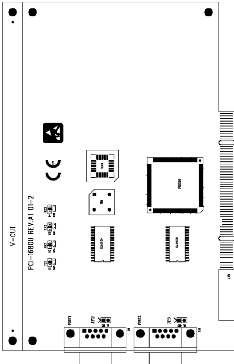
Figure 3.1 PCI-1680U Silk Screen
