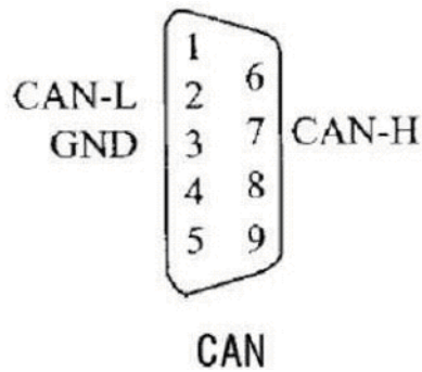
Figure 5.1 PCI-1680U/1682U DB-9 pin assignment
