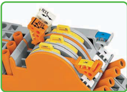
Lock-out has "snap" action into two notched positions preventing accidental operation of the disconnect link.
