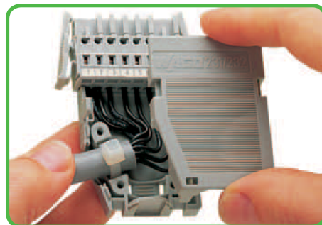
Snapping on the strain relief housing, demonstrated with a female connector with locking levers. Cable exits laterally. Strain relief by cable tie (up to a width of 4 mm).
