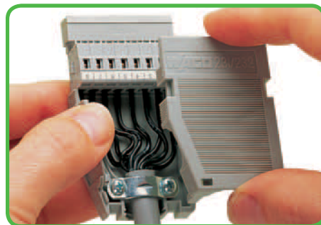
Snapping on a strain relief housing, demonstrated with a male connector. Cable exits lengthwise. Strain relief by cable clamp.
