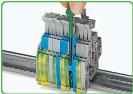
Removing a terminal block from the assembly.
