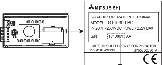
Example nameplate (manufacture's serial number 1010001)
