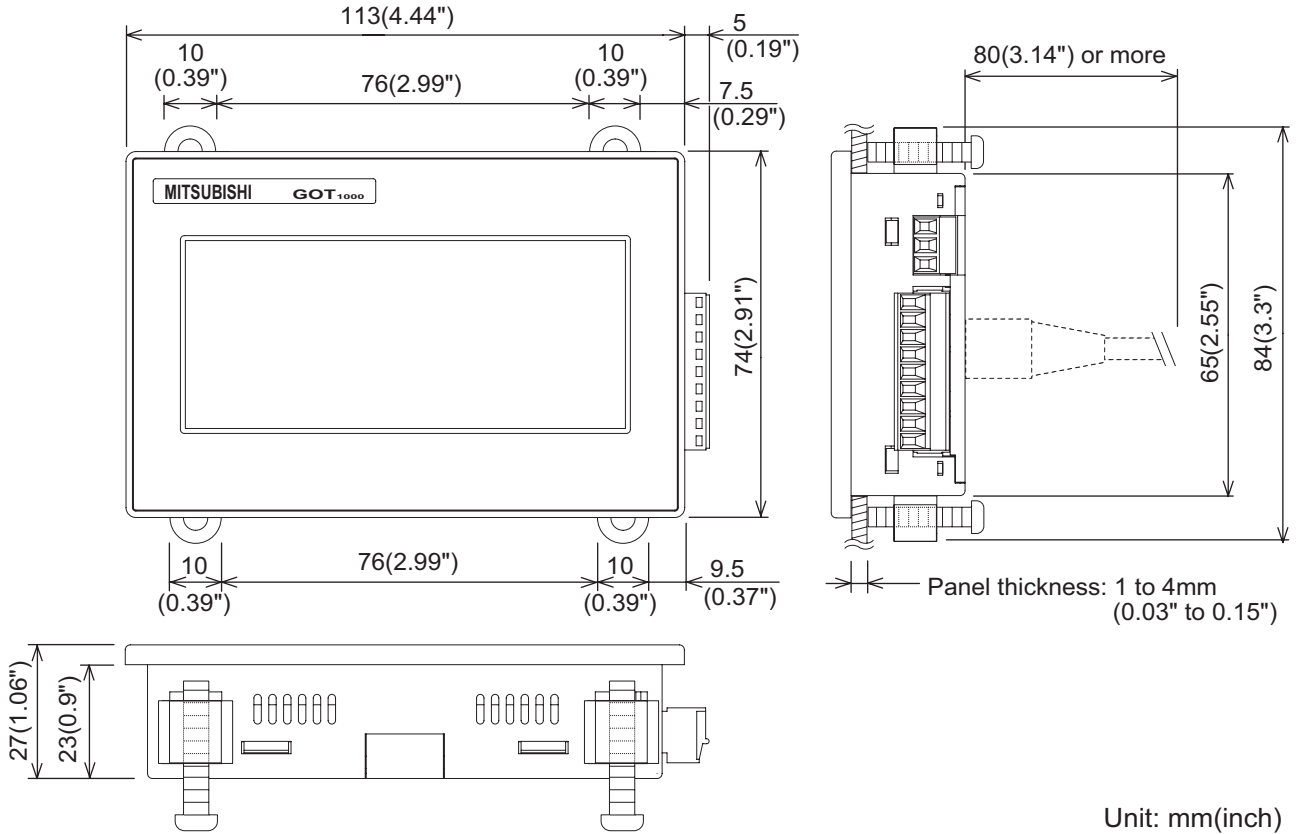
External dimensions of GT1020
