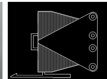
Side Latch
