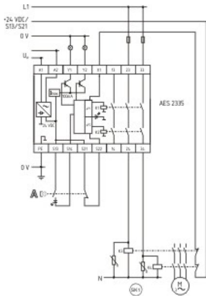
Wiring example
