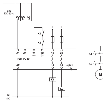
Circuit diagram
