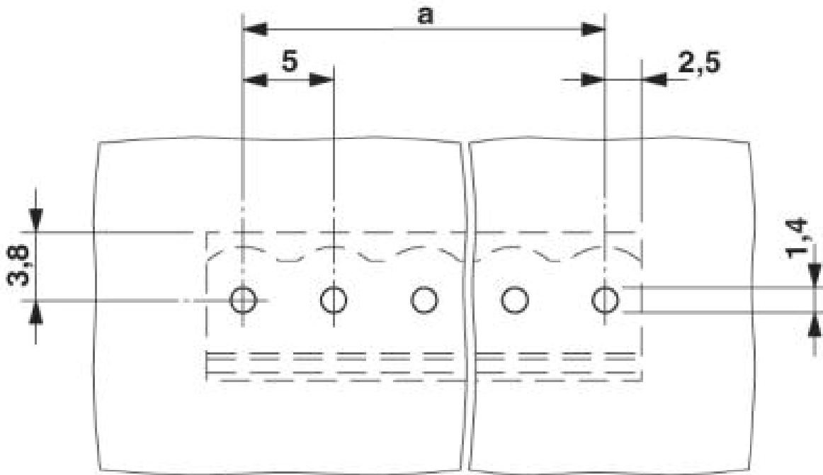
Drilling diagram
