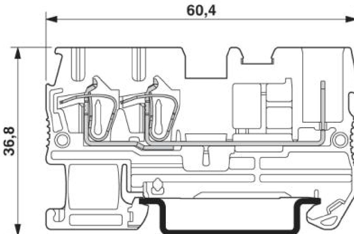
Dimensioned drawing
