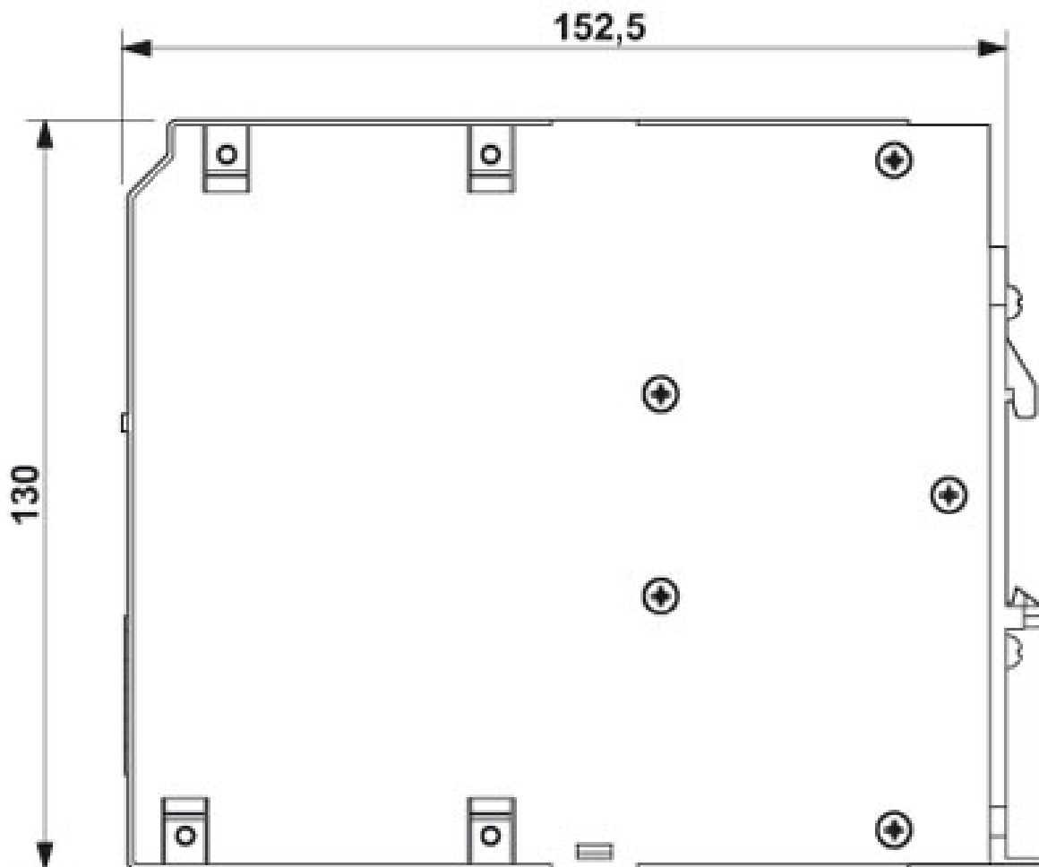
Dimensioned drawing
