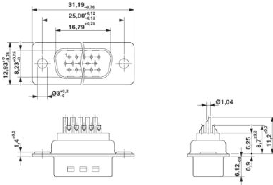
D-SUB contact insert
