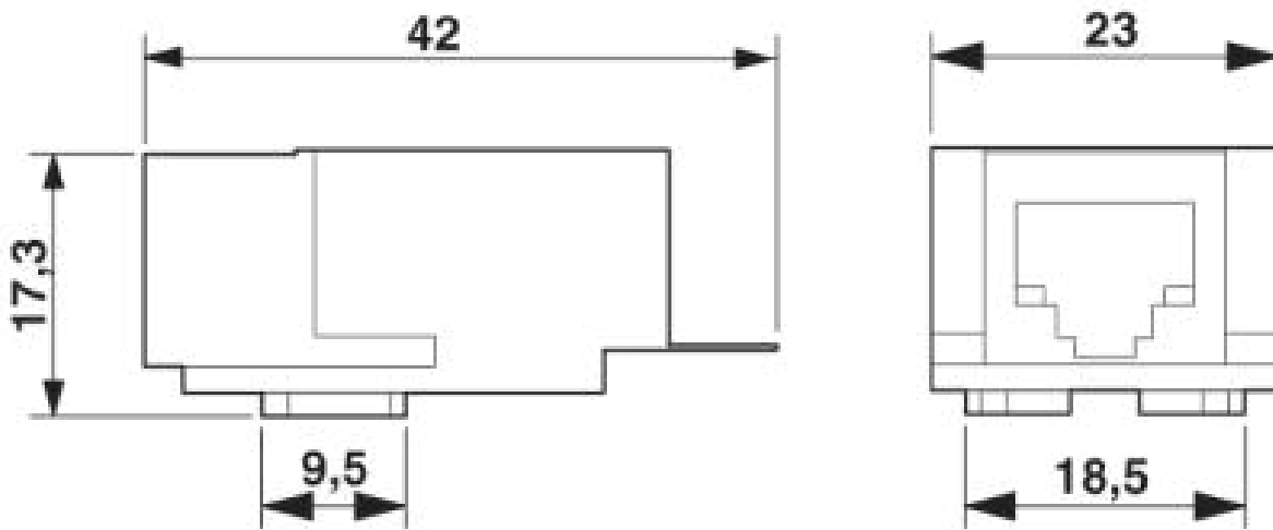
RJ45 socket insert
