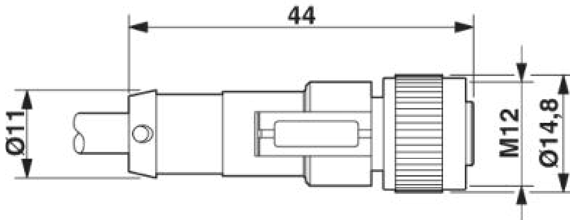
M12 x 1 socket, straight
