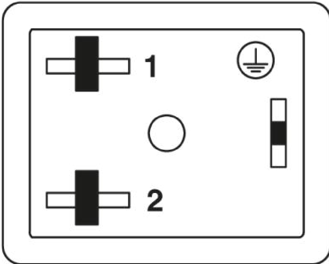
Valve connector pin assignment, type BI
