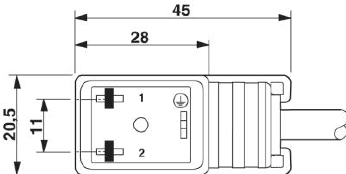
Valve connector, type BI
