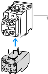
1 Contactor
